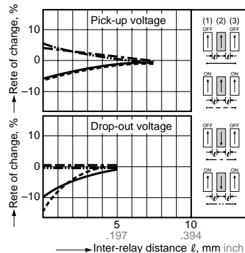
6-(1). Influence of adjacent mounting (1 Form C)
